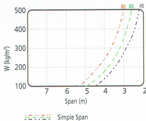
SIMPLE SUPPORT
